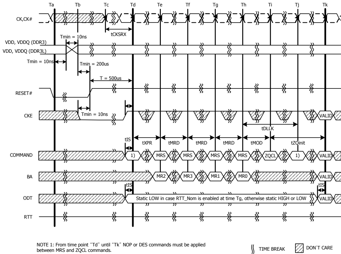
Figure 0 - VDD/VDDQ Voltage Switch Between DDR3L and DDR3
